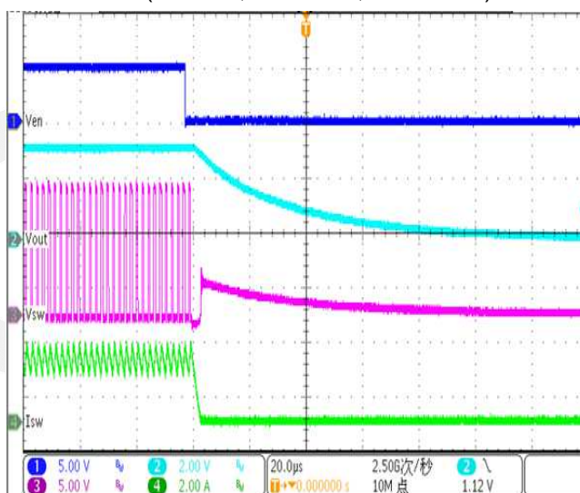
Shut down from Enable (V IN =12V, V OUT =3.3V, Load=1.5Ω)
